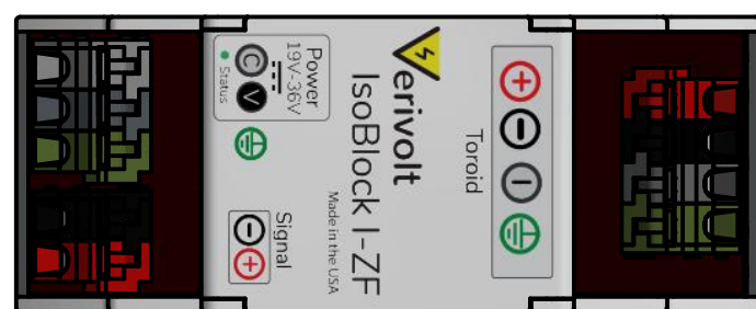
IsoBlock I-ZF SCALE 1 : 1
